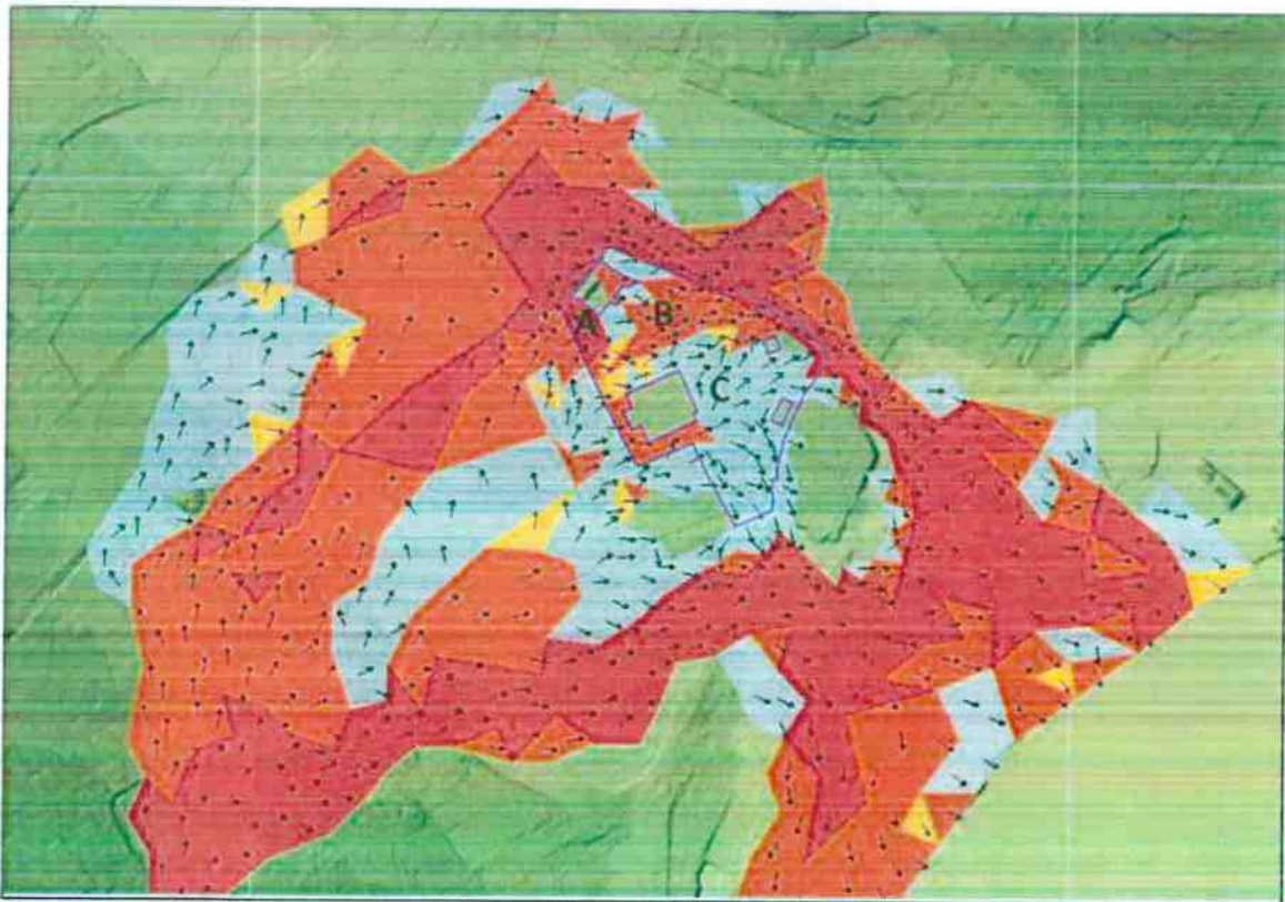
Plate 8.6: 2D model of reservoir inundation with maximum flood hazard values post-development
