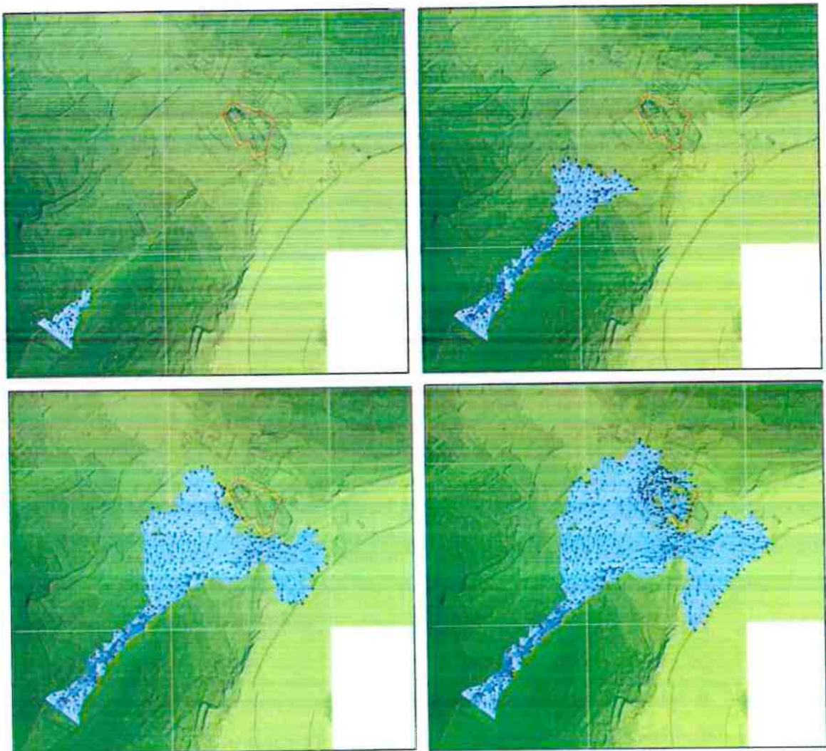
Plate 8.1: Time series (4min, 12min, 18min and 24min) of reservoir inundation flood event
