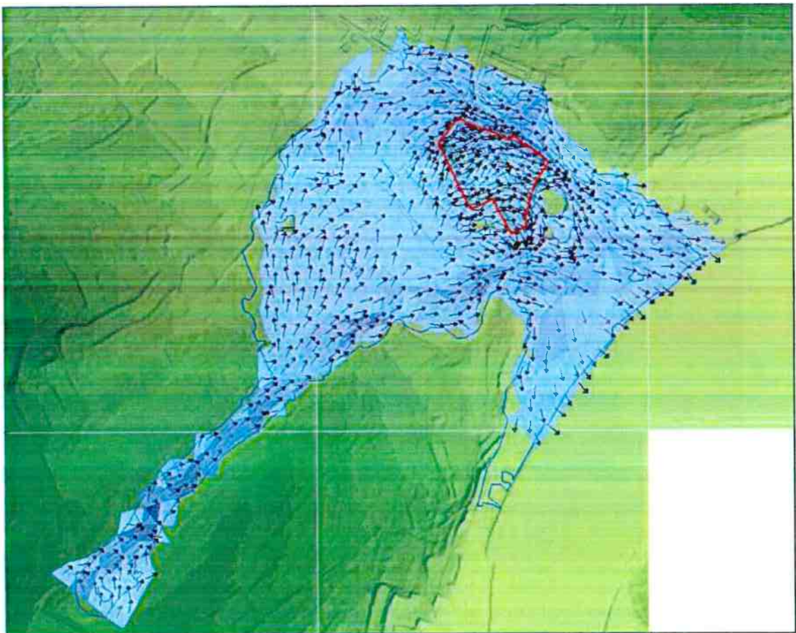
Plate 8.3: Maximum flood extent and depths resulting from a design flow with a peak of 1,000\text{m}^3/\text{s}
