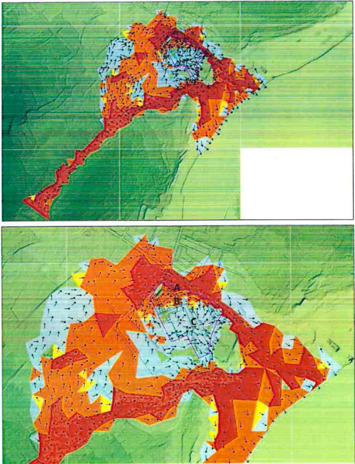
Plate 8.4: 2D model of reservoir inundation with maximum flood hazard values
